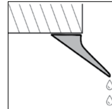
Polyprofil drip strip T60 on the underside of a balcony slab
