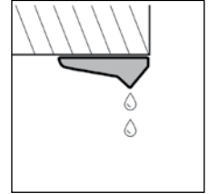
Polyprofil drip strip S40 on the underside of a balcony slab
